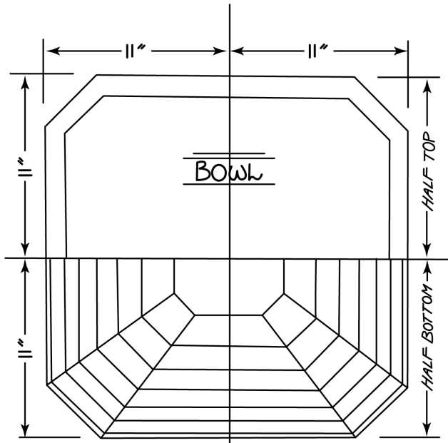
HALF PLAN-TOP & BOTTOM VIEW OF BIRD-BATH OR FOUNTAIN BOWL
