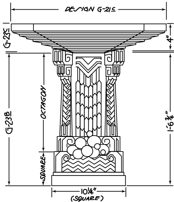
BIRD-BATH OR FOUNTAIN-SHOWING DESIGN G-23B & G-23C ASSEMBLY DESIGN G-23
