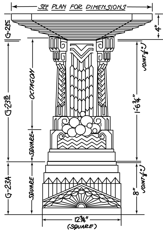
BIRD-BATH OR FOUNTAIN-SHOWING DESIGN G-23A, G-23B & G-23C ASSEMBLY DESIGN G-23
