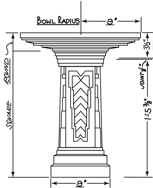
BIRD-BATH DESIGN G-24
